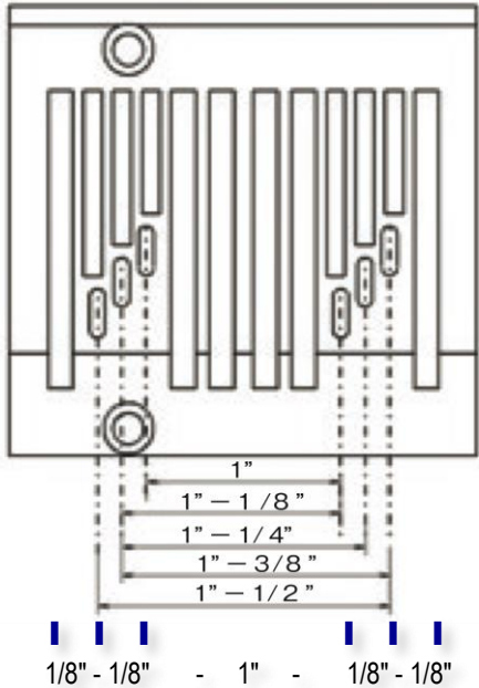
Split type presser foot
