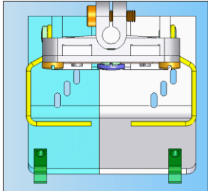
Split type presser foot
