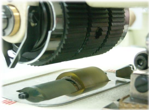
Gear iron upper puller and split type rubber lower puller
